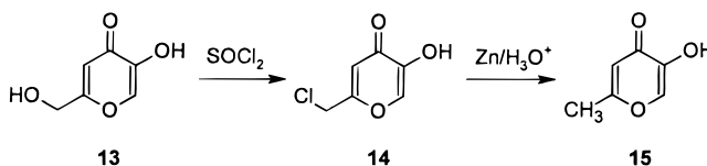
Scheme 4. Synthesis of 2-(1'-Hydroxyalkyl)-3-hydroxypyran-4-ones 16a–16e
