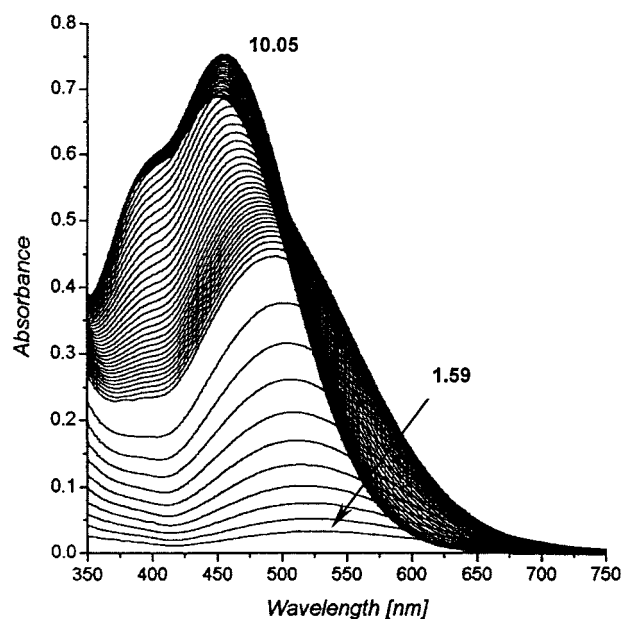
Figure 1. pH dependence of the spectrum of ligand 3 in the presence of iron(III) over the pH range 1.59–10.05: [Fe(III)] = 1.8 \times 10^{-4} M; [ 3 ] = 1.8 \times 10^{-3} M.
