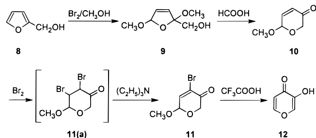
Scheme 2. Synthesis of Pyremeconic Acid ( 12 ) from Furfuryl Alcohol
