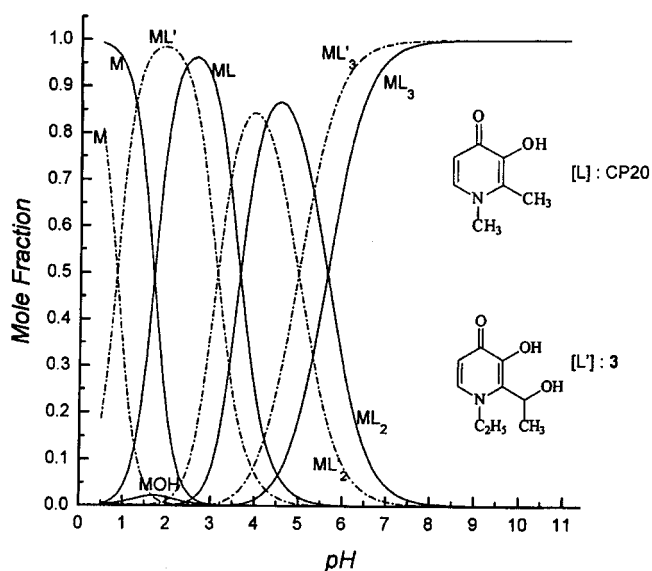
Figure 3. Comparison of the speciation plots between CP20 and 3 in the presence of iron(III): L = CP20; L' = 3 ; [\text{Fe(III)}] = 1 \times 10^{-6} \text{ M} ; [\text{ligand}] = 1 \times 10^{-5} \text{ M} .
